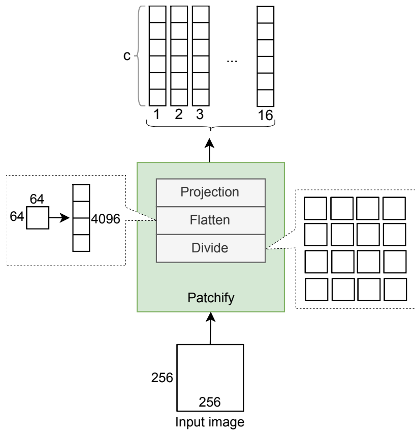
Figure 9: Patchification process
